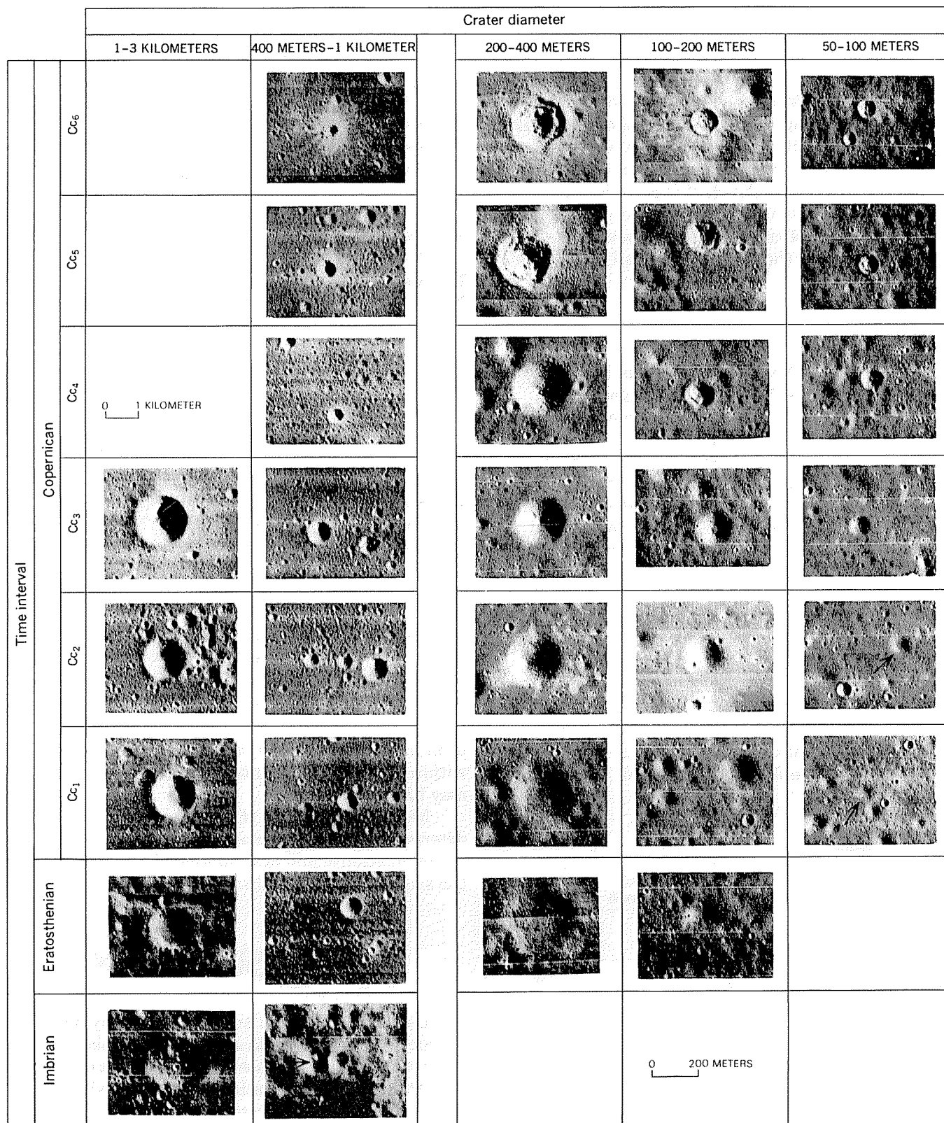
FIGURE 7.12.—Craters smaller than 3 km in diameter, arrayed by age and size. Sun-illumination angles are mostly 19.5^\circ above horizontal; a few are from 18.2^\circ to 23^\circ . Craters of each size decrease in sharpness with age. From Trask (1971, fig. 2).
